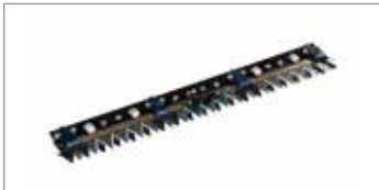
Complete central cutter plate 1.15 m Special teeth Side protection discs Code 69229069A
