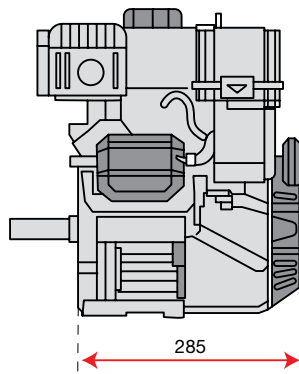
Engine p/n 3075210
