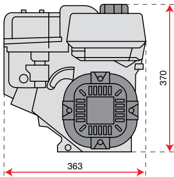
Engine p/n 3075069
