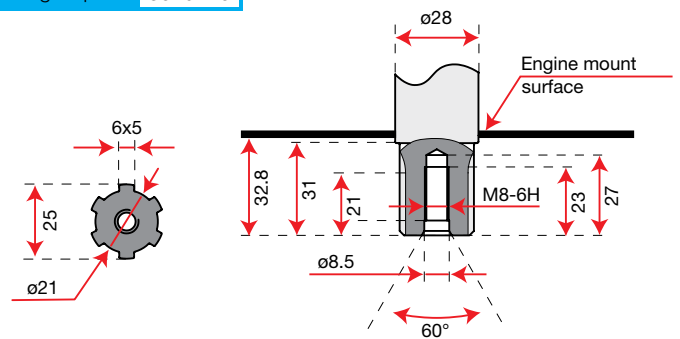
Engine p/n 3075210
