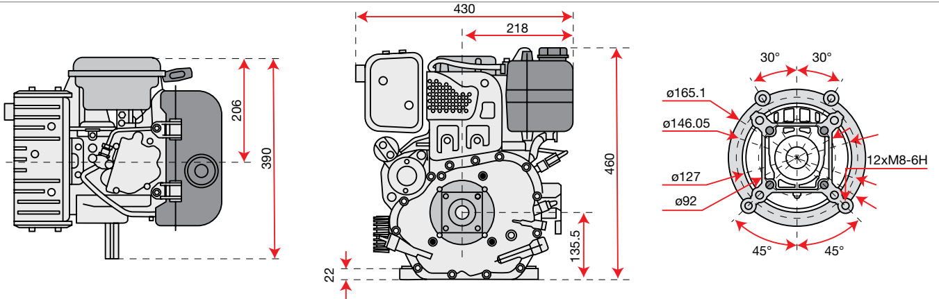
Engine p/n 3175016A
