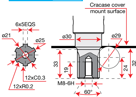
Engine p/n 3175016A
