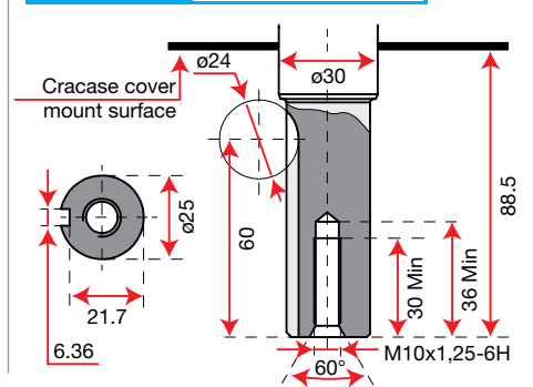
Engine p/n 3175000* - 3175019A
