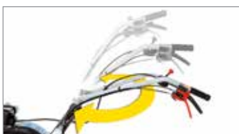
Handlebars with horizontal and vertical adjustment to allow the operator to assume the correct posture while working.
