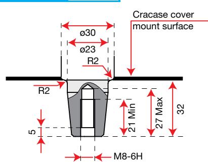
Engine p/n 3175031
